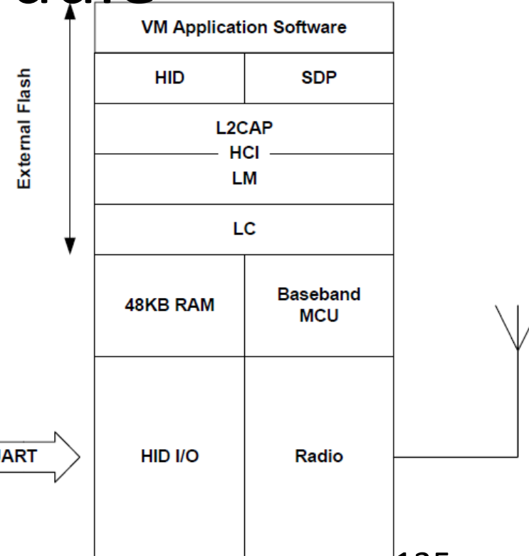
Figure 9.4: HID Stack
