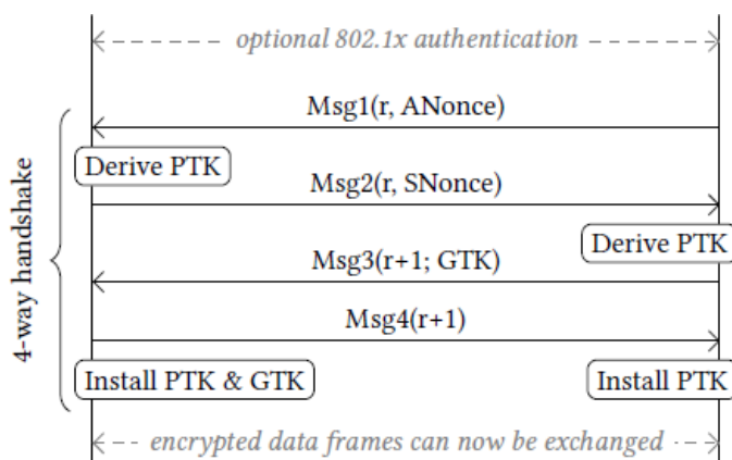
IEEE 802.11 Four Ways Handshake
