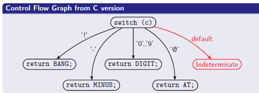
Exemple de graphe CFG ( Control Flow Graph )
